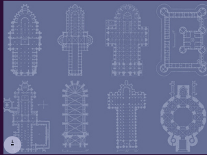
Architecture Complexity
